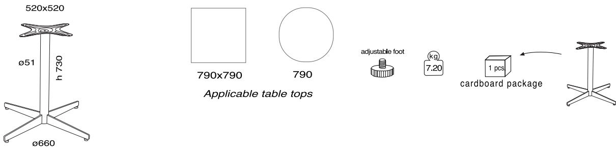
Gala 341 Table base
